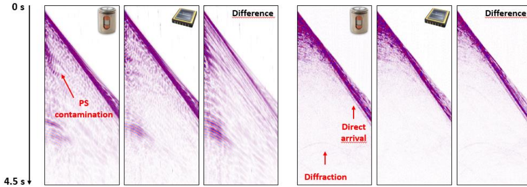
Figure 1: Example of Z (vertical) CRG in m/s: 16-32 Hz (left) and 64-128 Hz (right) bandpass filter.
