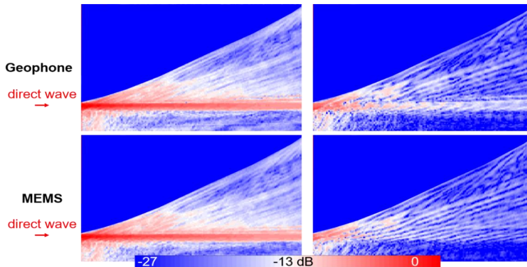
Figure 2: Signal envelopes in dB (m/s) for the geophone data (top) and MEMS data (bottom). (X,Y,Z) envelope (left), and (Z) envelope (right).
